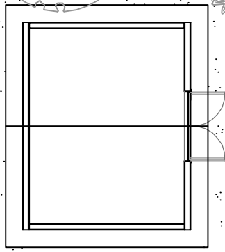
SHED PLAN 'LAYOUT -1'
